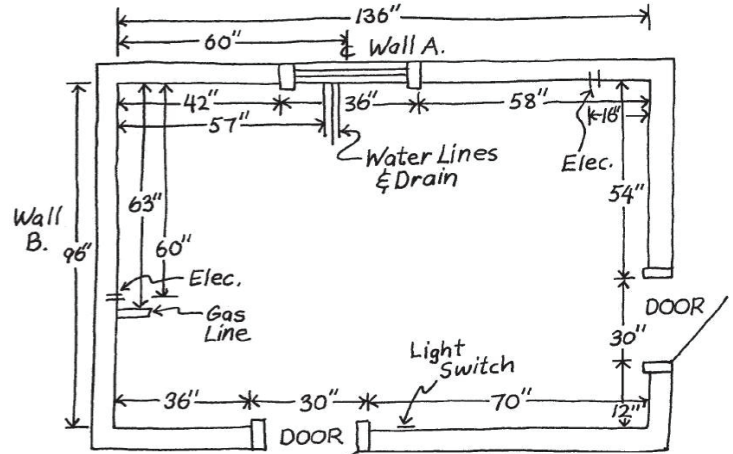
Example Floor Plan
